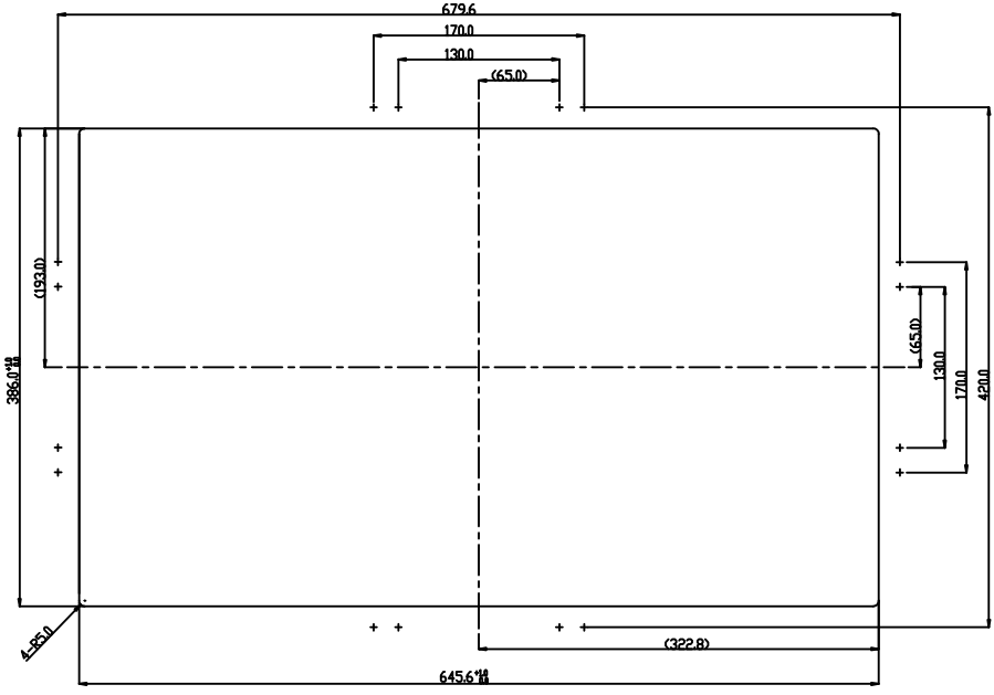
RECOMMENDED CUSTOMER PANEL CUT-OUT(REAR MOUNT)
