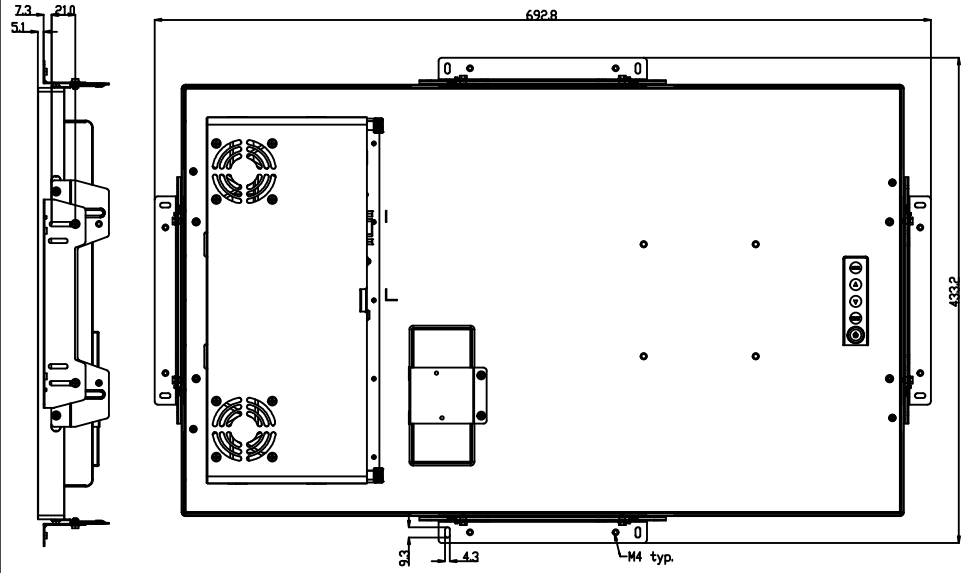
REAR MOUNT WITH BRACKETS, HORIZONTAL OR VERTICAL
